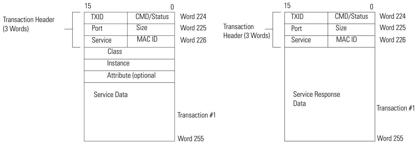
Format of 32-word M0 Transfer File for Explicit Message Request
