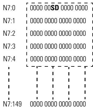
SLC 500 Processor Input Data File 1
