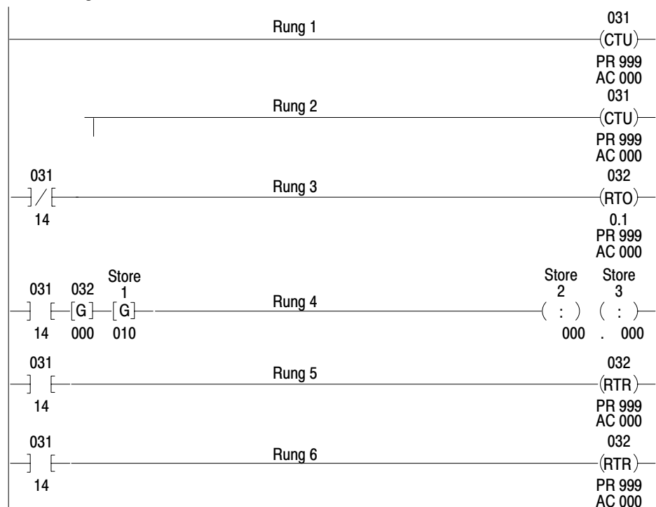
Figure 8.2 Average Scan Time
