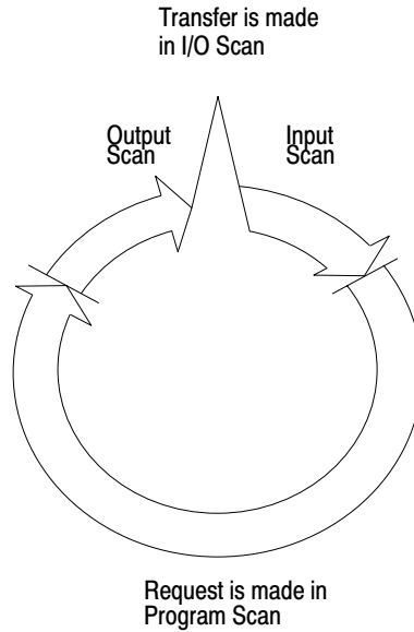
Figure 18.2 Block Transfer Timing Diagram
