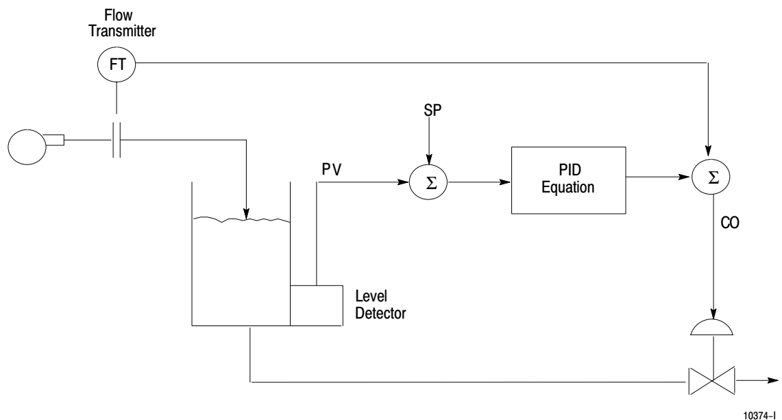
Figure 16.9 This is an Example of Feedforward Control
