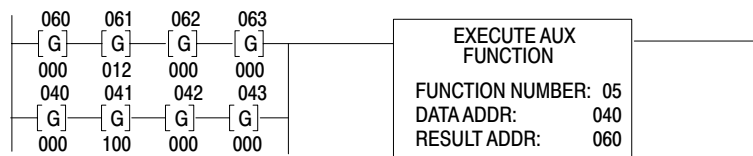
Figure 14.12 EAF Input and Result Rung
