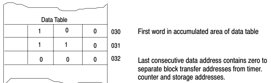
Figure 18.4 Defining the Data Address Area
