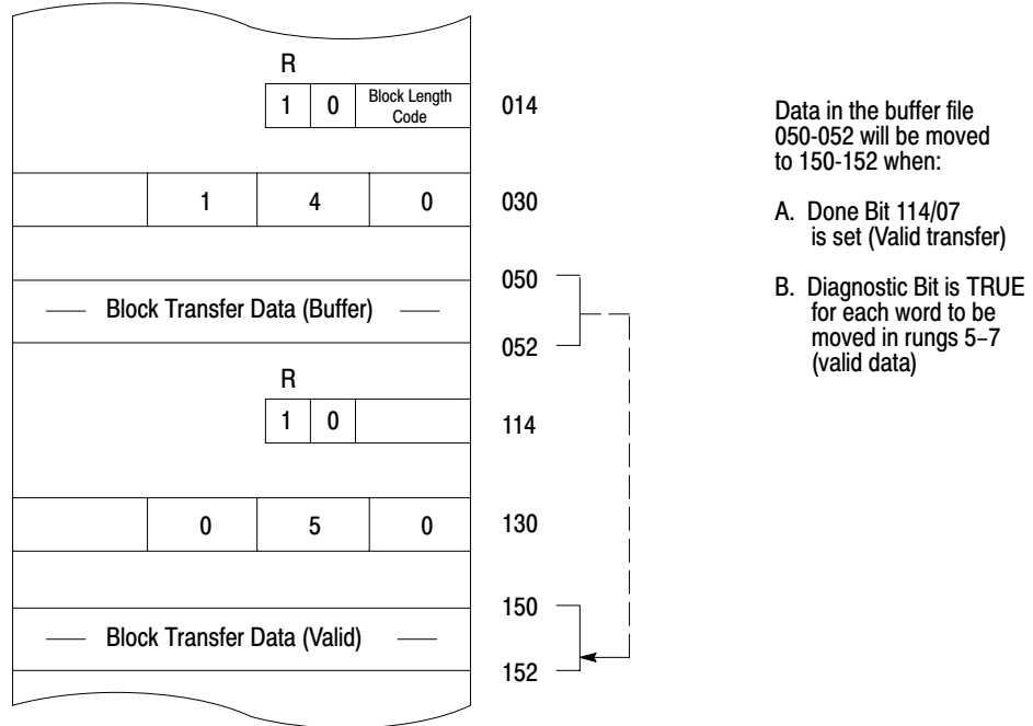
Figure 18.8 Buffering Data
