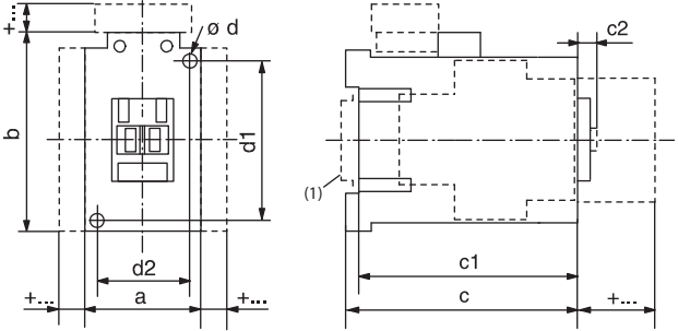
(1) May be mounted to 35 mm EN 50 022 DIN Rail.
