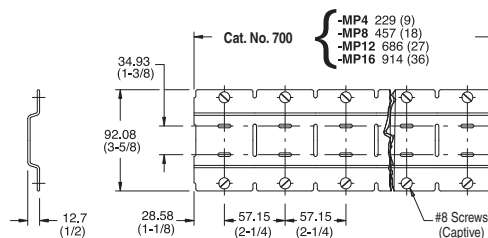
Relay Rail for 700-P, -N, -NM, -R, -RM, -RT, -RTA Relays Secure the mounting strip with two screws at each end relay position. Use a minimum of one screw at the 3rd, 5th, 7th, etc., relay positions. Alternate between upper and lower horizontal slots.
