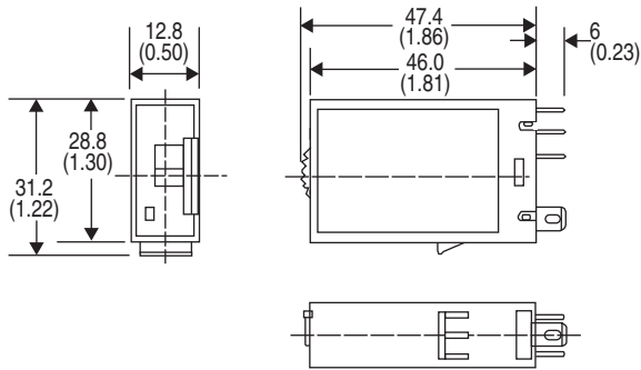
700-HNK41 SPDT Contact
