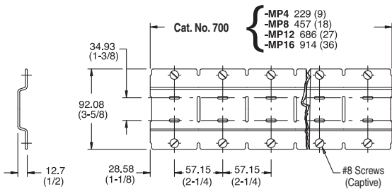
Relay Rail
