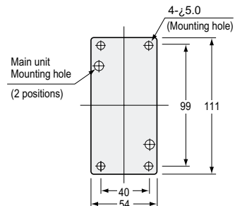
Mounting bracket OP-35345
