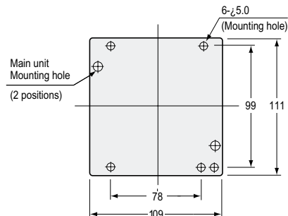
Mounting bracket OP-35348
