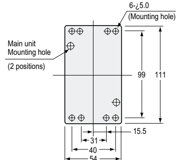
Mounting bracket OP-35346
