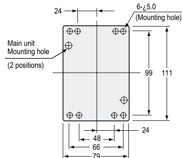
Mounting bracket OP-35347
